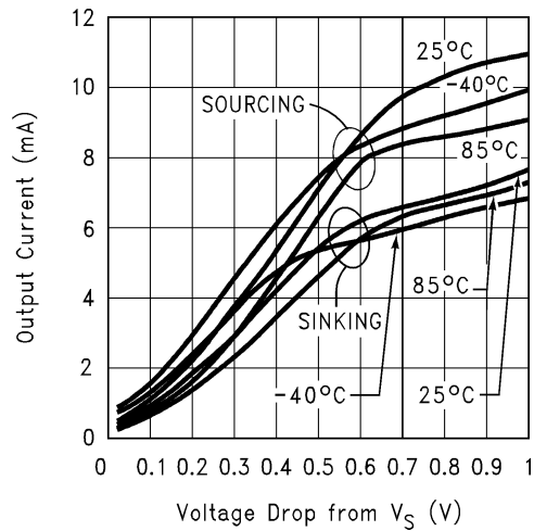
V_O vs I_O , V_S = \pm 1.1\text{V}
