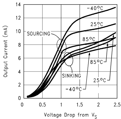
V_O vs I_O , V_S = \pm 2.5\text{V}
